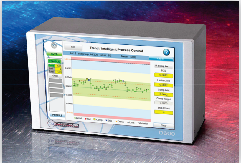
D600 Gage Controller with IPC Trend Page displayed
